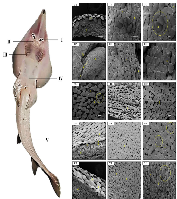
Figure 4: Photomicrography of P. horkelli in ventral view, indicating the regions where the samples were collected and their respective photomicrographs by scanning electron microscopy, highlighting the circular morphology of the denticles in each region. In I ABC nasal cavity, II ABC preoral region, III ABC region of the branchial clefts, IV ABC abdominal region ventral side and V ABC caudal region ventral side. The dermal denticle (a), epithelium (b), preoral sulcus (c), muscular layer with rectangular bundles (d), central cavity and pulp of the denticle (e) are evident.
